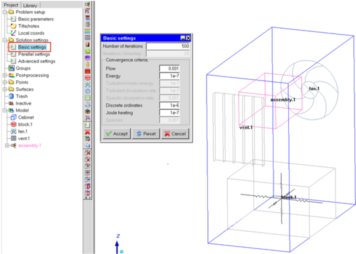
Figure 3-12: Classic Icepak Basic Settings
