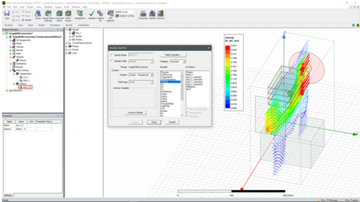
Figure 3-30: Icepak Field Plot - Velocity Vectors Plane Cut
