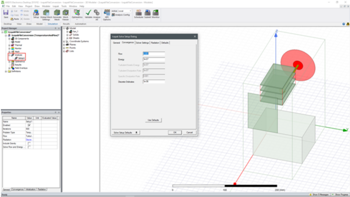
Figure 3-21: Icepak Solve Setup Dialog - Convergence Tab
