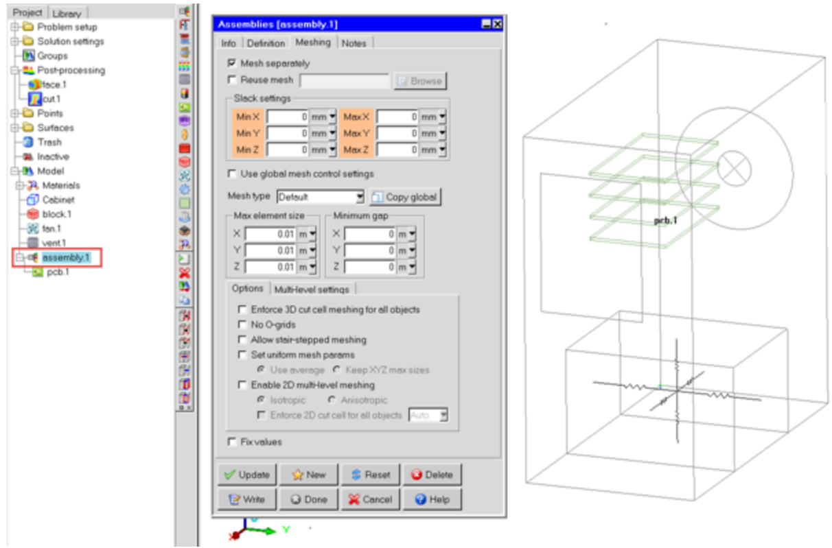
Figure 3-8: Classic Icepak Assembly Meshing Options
